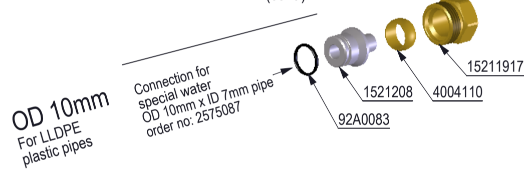
UNIFLEX CONNECTIONS IN STAINLESS STEEL FOR LLDPE PLASTIC PIPE (cont.)
