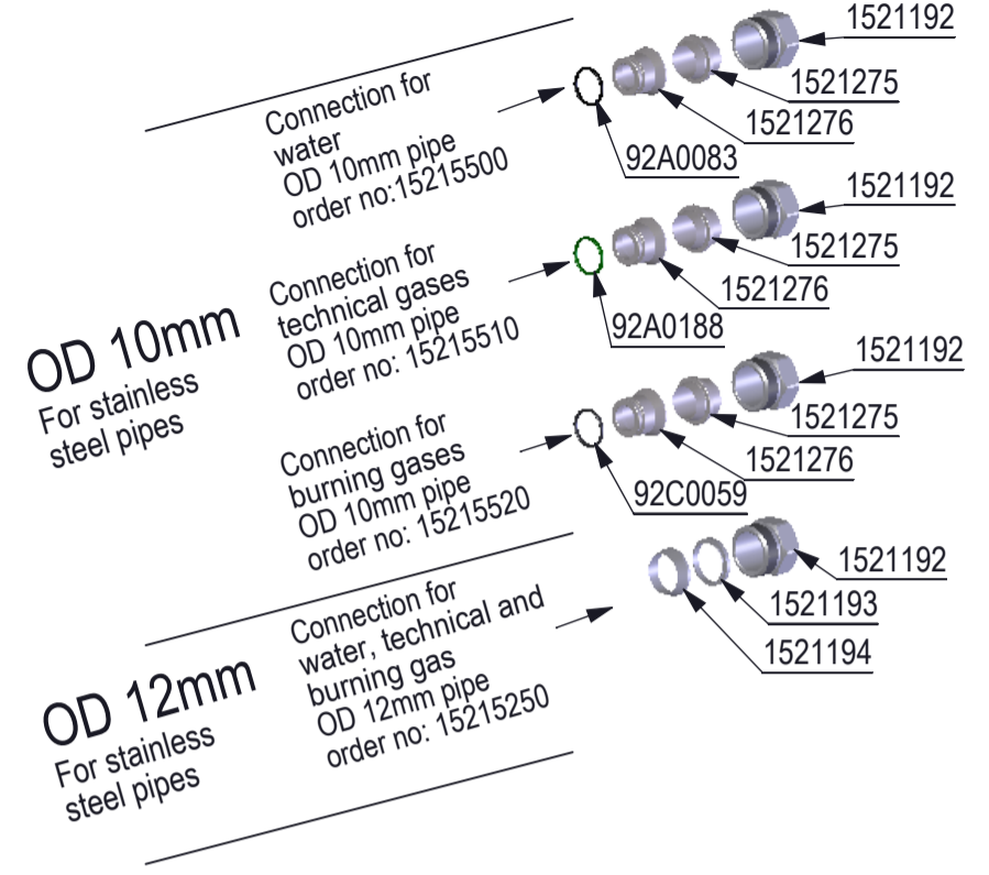
UNIFLEX CONNECTIONS FOR STAINLESS STEEL PIPES (cont.)
