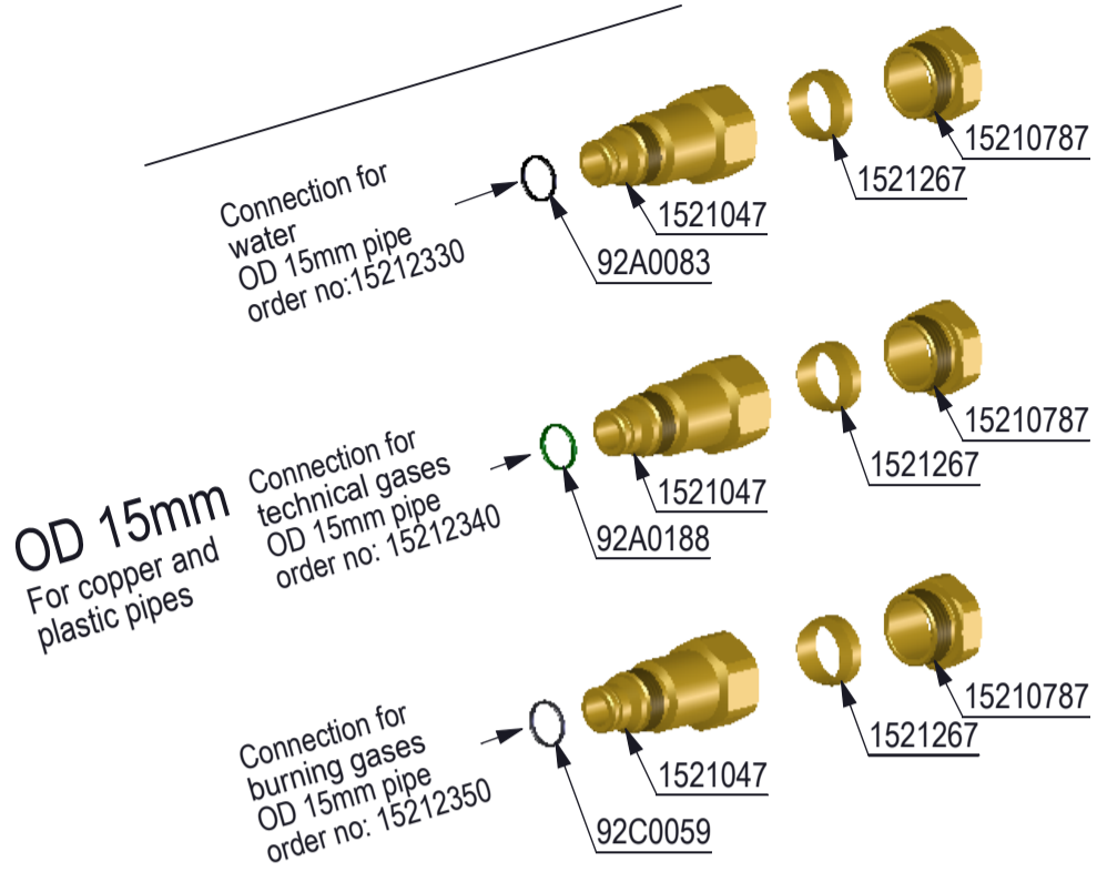
UNIFLEX CONNECTIONS FOR COPPER AND PLASTIC PIPES (cont.)
